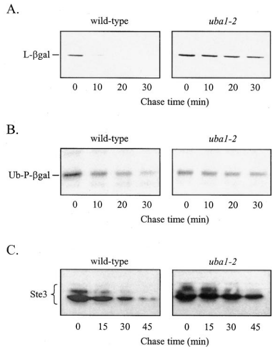
Fig. 4. uba1-2 is impaired in a variety of ubiquitin related processes. A: Pulse-chase analysis of degradation of Leu-βgal in wild-type and uba1-2 cells. B: Pulse-chase analysis of degradation of Ub-Pro-βgal in wild-type and uba1-2 cells. C: Immunoblot analysis of Ste3 degradation in wild-type and uba1-2 cells. Protein synthesis was blocked at t =0 min by addition of 50 μg/ml cycloheximide.
